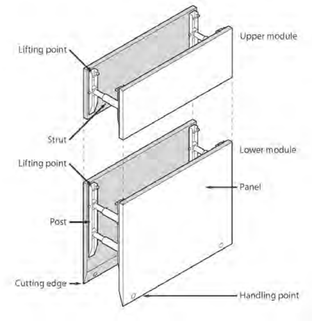
Figure 19: Typical trench shield
