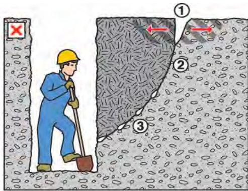
(a) This is a very dangerous situation, requiring ground support. No worker should be in a trench > 1.5m deep unless support has been installed.
