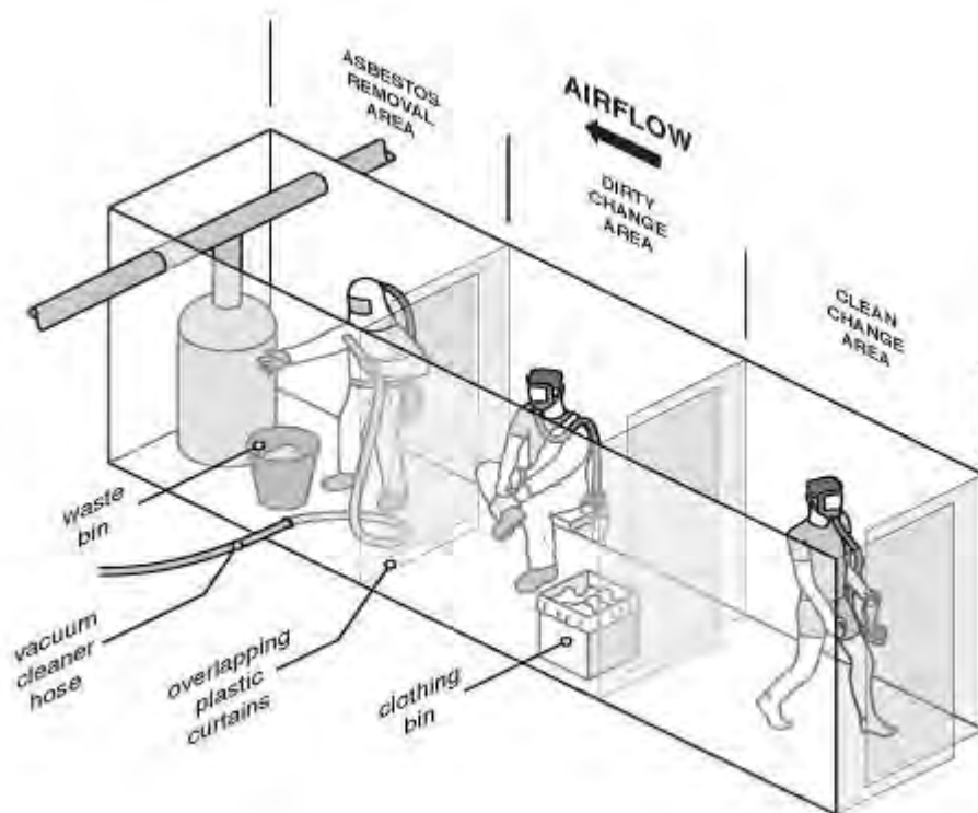
Figure 2: Decontamination area.
