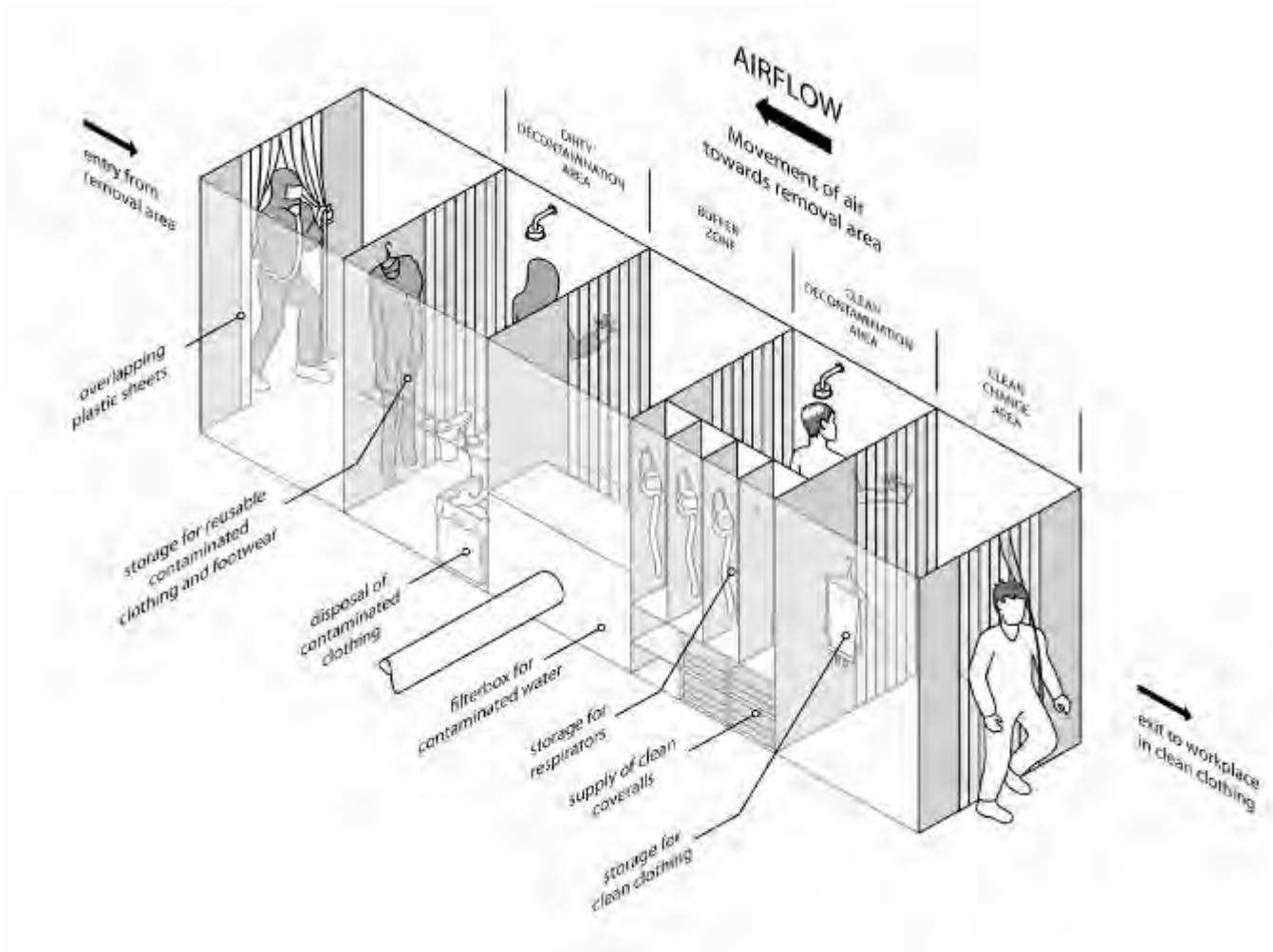
Figure 1: Decontamination unit.
